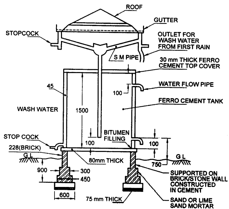
WATER TANK ABOVE GROUND
