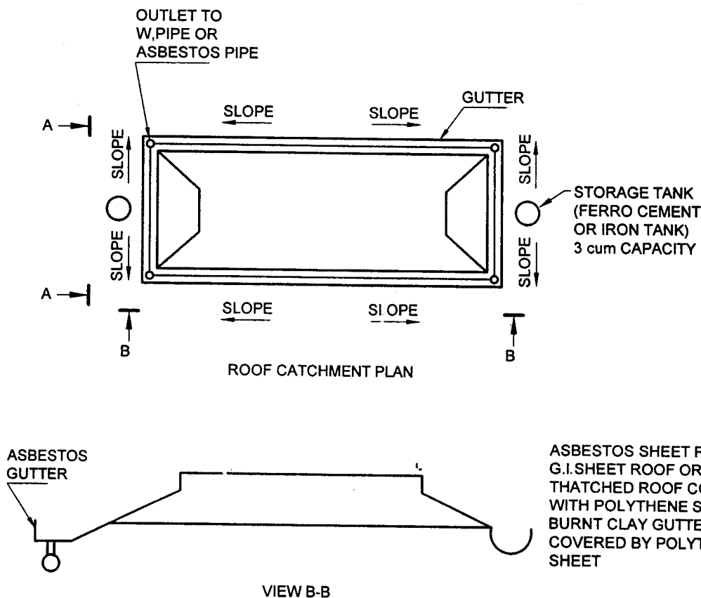
FIG. 1 RAINWATER HARVESTING SYSTEM
