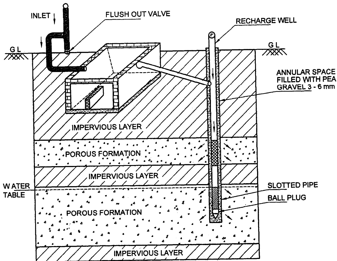
FIG. 7 RECHARGE THROUGH BORE WELL
