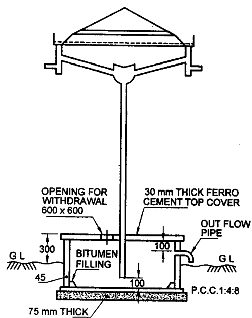
WATER TANK UNDER GROUND
