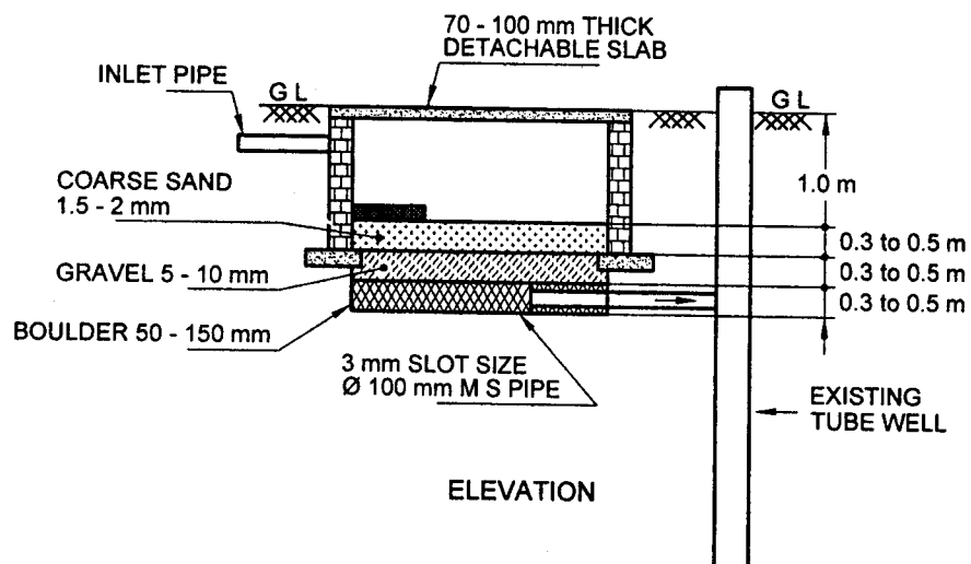
FIG. 6 RECHARGE THROUGH EXISTING TUBE WELL
